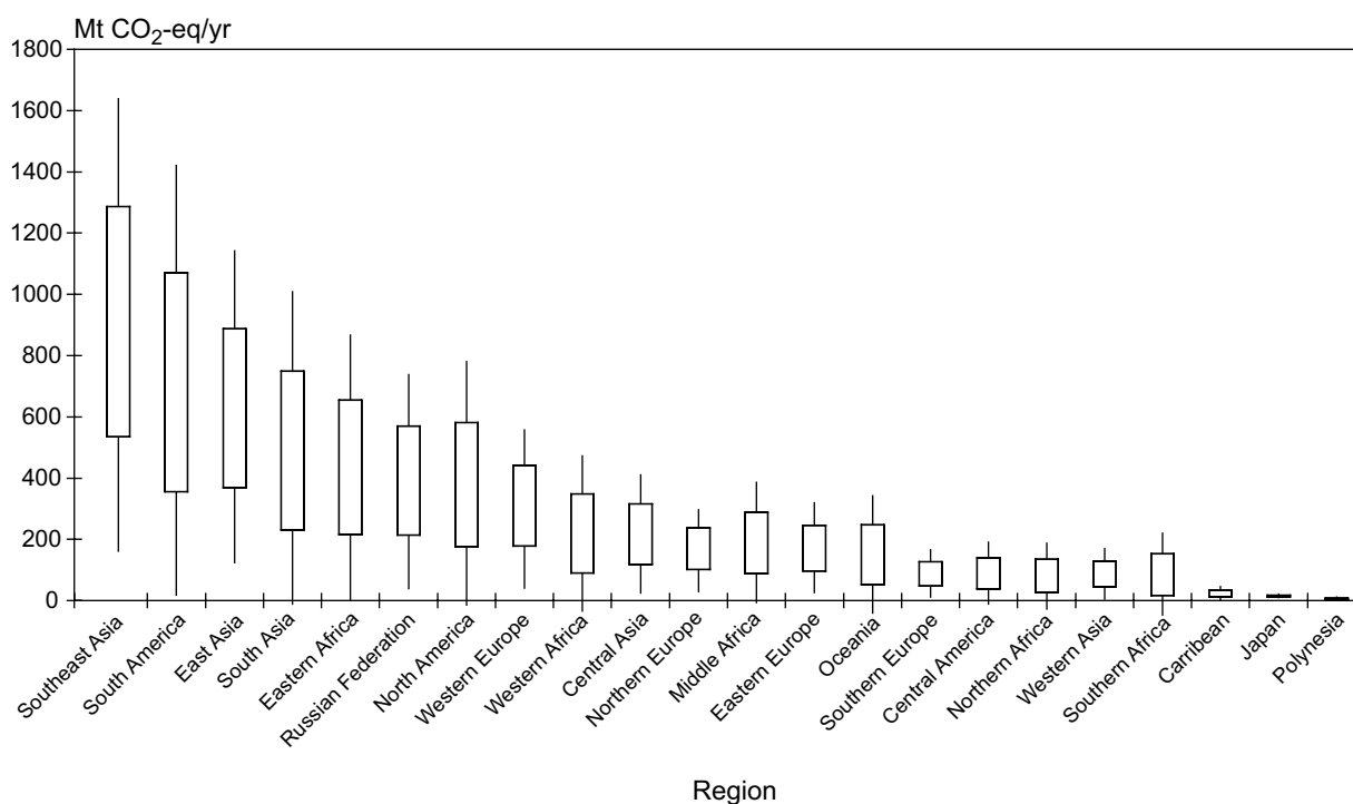
Figure 8.6: Total technical mitigation potentials (all practices, all GHGs) for each region by 2030
