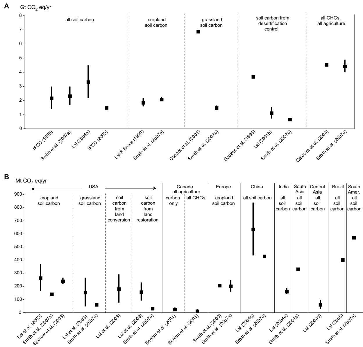
Figure 8.3: Global (A) and regional (B) estimates of technical mitigation potential by 2030 Note: Equivalent values for Smith et al. (2007a) are taken from Table 7 of Smith et al., 2007a.
