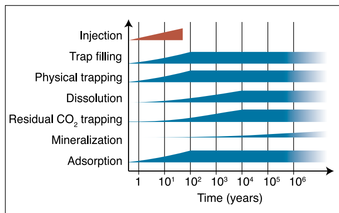
Figure 5.18 Schematic showing the time evolution of various \text{CO}_2 storage mechanisms operating in deep saline formations, during and after injection. Assessing storage capacity is complicated by the different time and spatial scales over which these processes occur.
