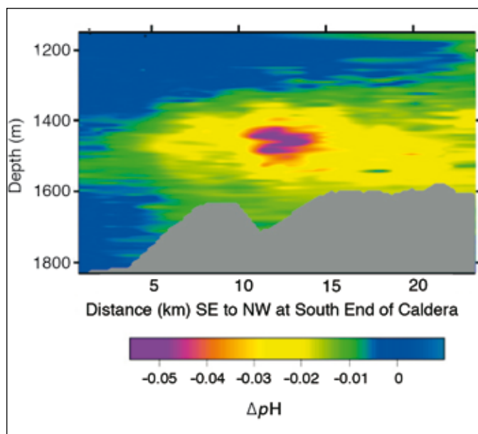
Figure 6.23 Measurements showing the ability to measure chemical effects of a natural \text{CO}_2 plume. Profiles for \text{pH} were taken in June 1999 near the Axial Volcano at 46^\circ\text{N} 130^\circ\text{W} , in the ocean near Portland, Oregon, United States.
