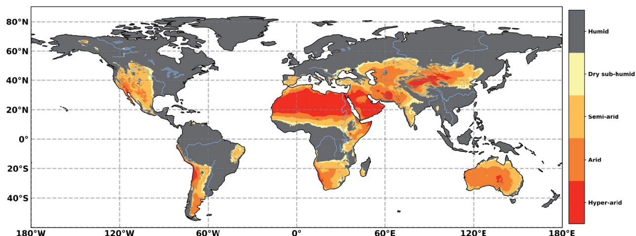
Figure TS.6 | Geographical distribution of drylands, delimited based on the aridity index (AI). The classification of AI is: Humid AI > 0.65, Dry sub-humid 0.50 < AI \leq 0.65 , Semi-arid 0.20 < AI \leq 0.50 , Arid 0.05 < AI \leq 0.20 , Hyper-arid AI < 0.05. Data: TerraClimate precipitation and potential evapotranspiration (1980–2015) (Abatzoglou et al. 2018).
